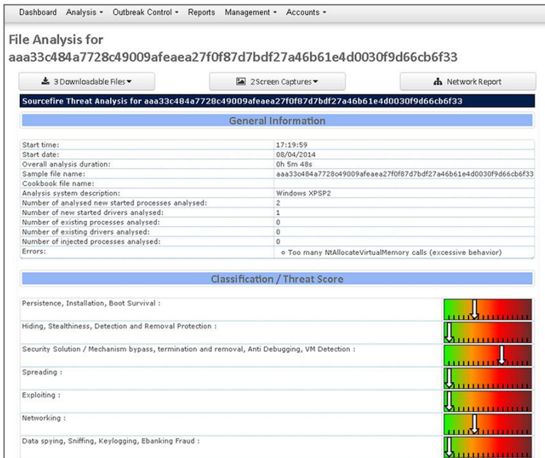
Figure 4. File Analysis
